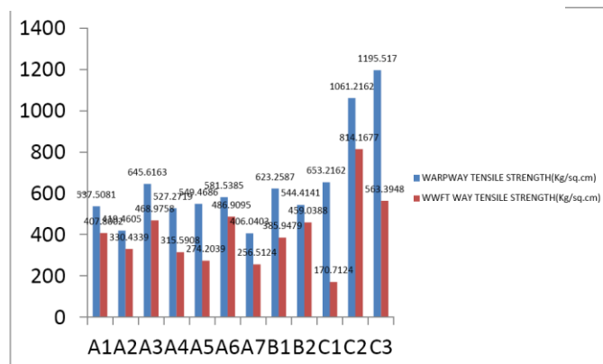
FIGURE 3.7 TENSILE STRENGTH OF FABRIC
