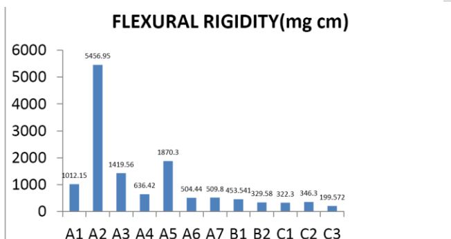
FIGURE 3.5 FLEXURAL RIGIDITY OF FABRIC
