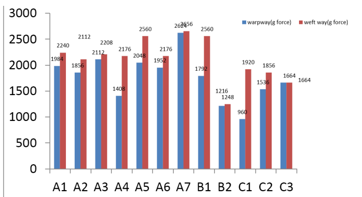
FIGURE 3.6 TEARING STRENGTH OF FABRIC
