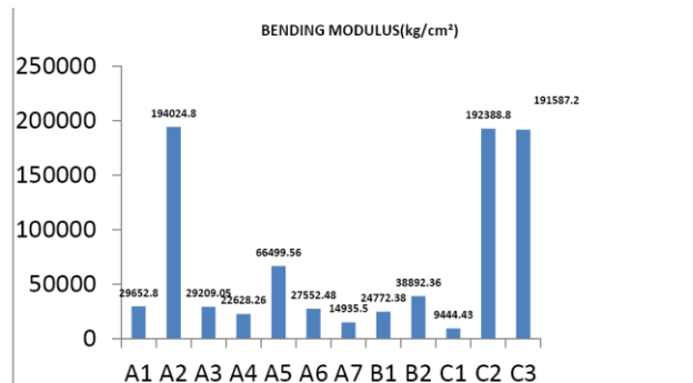
FIGURE 3.5 BENDING MODULUS OF FABRIC
