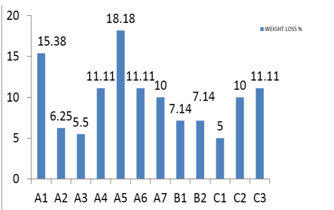
FIGURE 3.3 ABRASION RESISTANCE OF FABRIC
